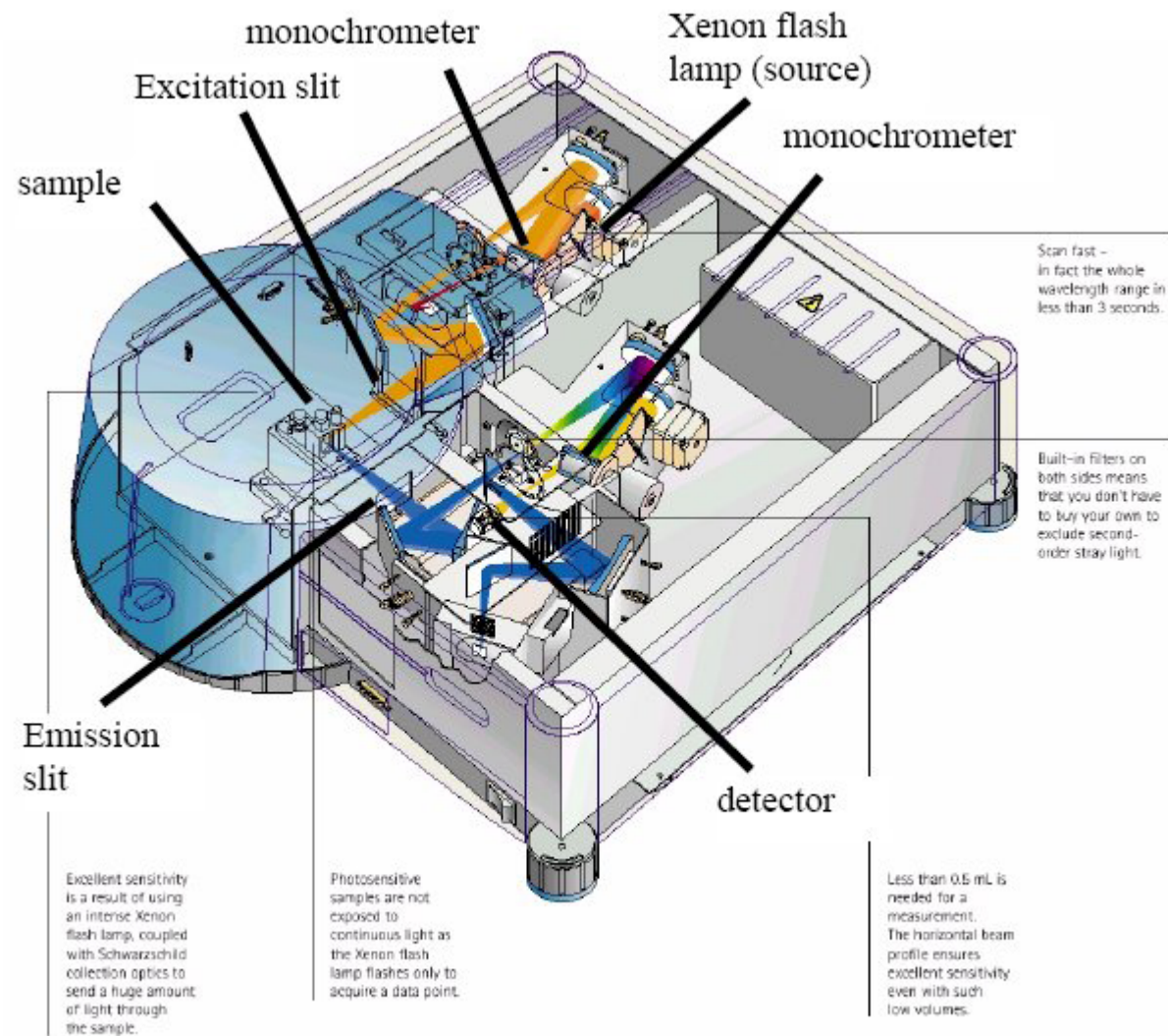
Fig. 1 The Cary Eclipse Fluorimeter
