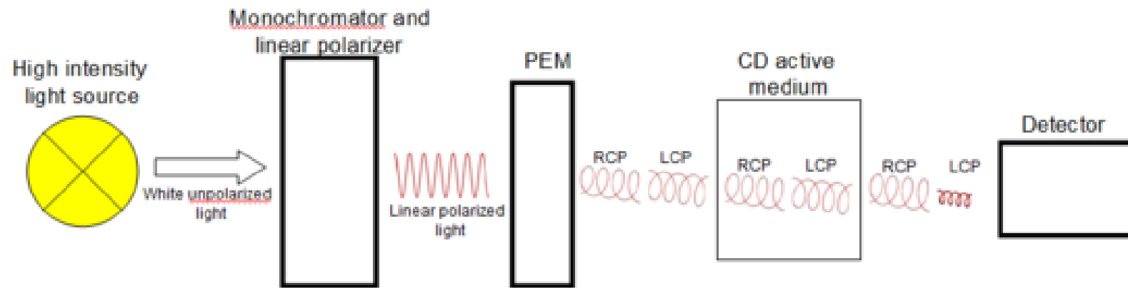
Photoelastic Modulator
